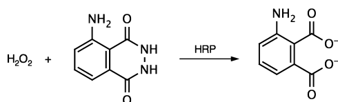
Figure 1. Luminescence reaction catalyzed by HRP.
